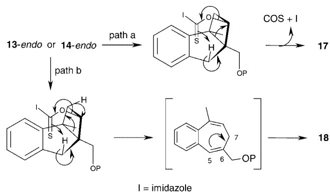
Figure 2. Mechanistic considerations of the formation of by-products 17 and 18 .
