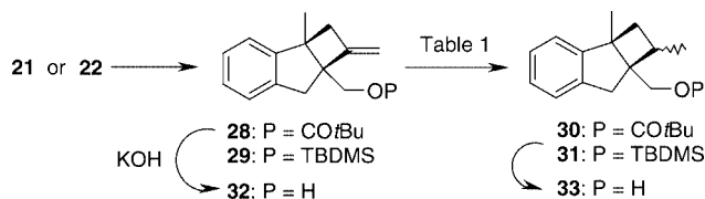
Scheme 8. 1-Substituted cyclobutanes based on Wittig chemistry.
