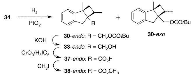
Scheme 11. Diastereoselectivity of the hydrogenation of 34 .
